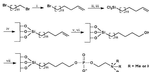
Scheme 1 The synthetic procedure for covalent bonding of an organic monolayer bearing terminal PC or PA groups. Reagents and conditions: i, allylmagnesium bromide, -10 to -20 °C; ii, Mg, THF, 20 °C; iii, \text{SiCl}_4 ; iv, silicon block, \text{CH}_2\text{Cl}_2 –hexadecane (1:4), 11 °C, 1.5 h; v, \text{BH}_3 ·THF, 10 min, 20 °C; vi, \text{H}_2\text{O}_2/\text{OH}^- ; vii, \text{POCl}_3 , \text{NEt}_3 , 10 to 20 °C.
